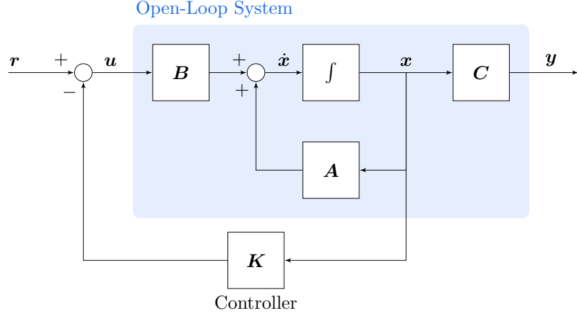
Figure 3.1: Block diagram of a state-feedback closed-loop system.
