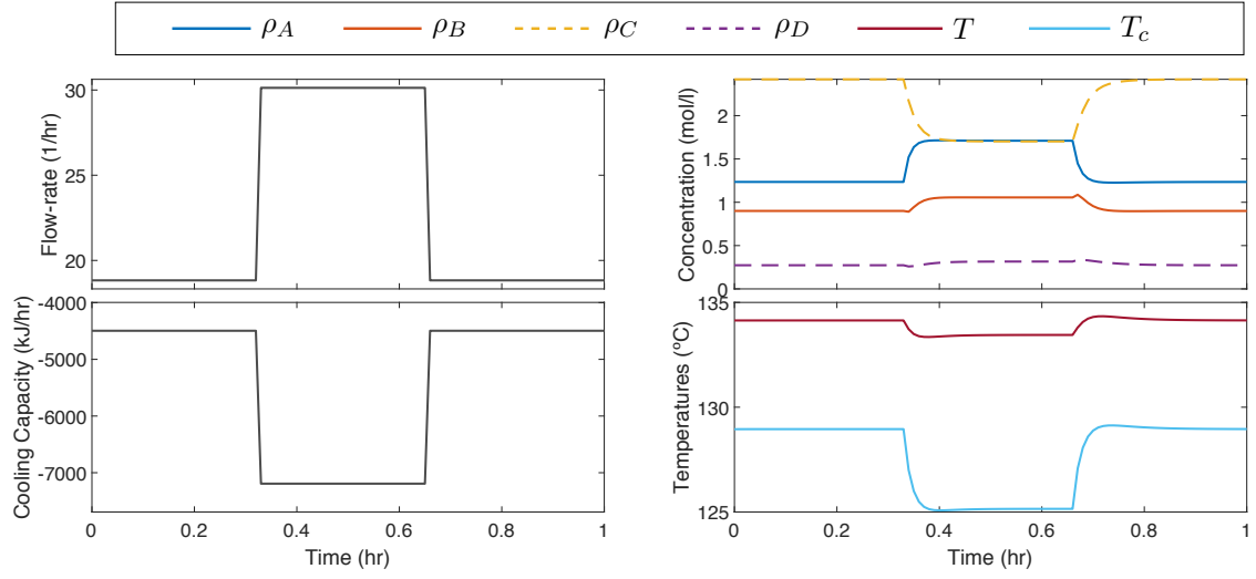
Figure 6.3: Non-linear simulation showing the manipulated variables (left) and correspondent response of the system variables (right) for a change in the input flow-rate and cooling capacity.
