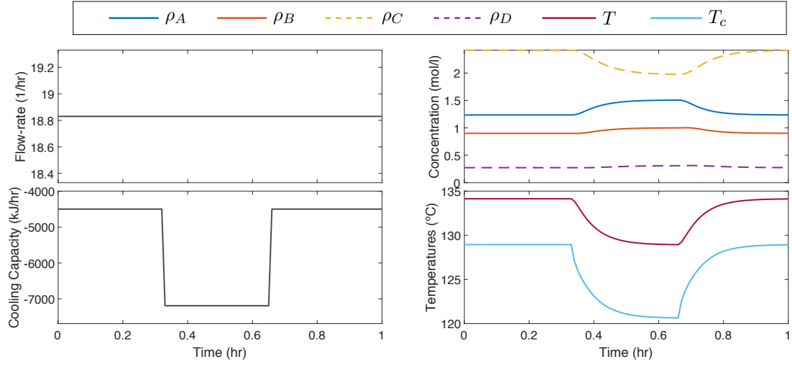
Figure 6.2: Non-linear simulation showing the manipulated variables (left) and correspondent response of the system variables (right) for a pulse change in the cooling capacity.
