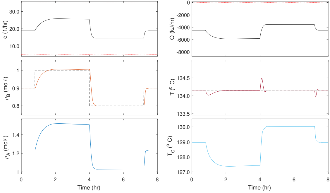
Figure 6.10: Simulation of the LQRI_1 for reference tracking.
