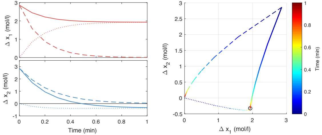
Figure 2.4: Simulation of the total response decomposition for the two first states of the model from (2.39). Each state response is shown separately (left) and together into a trajectory visualization (right), in which the steady-state point is indicated by a circle.
