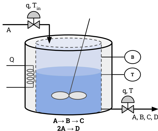
Figure 5.1: The non-isothermal continuous stirred tank reactor proposed.
