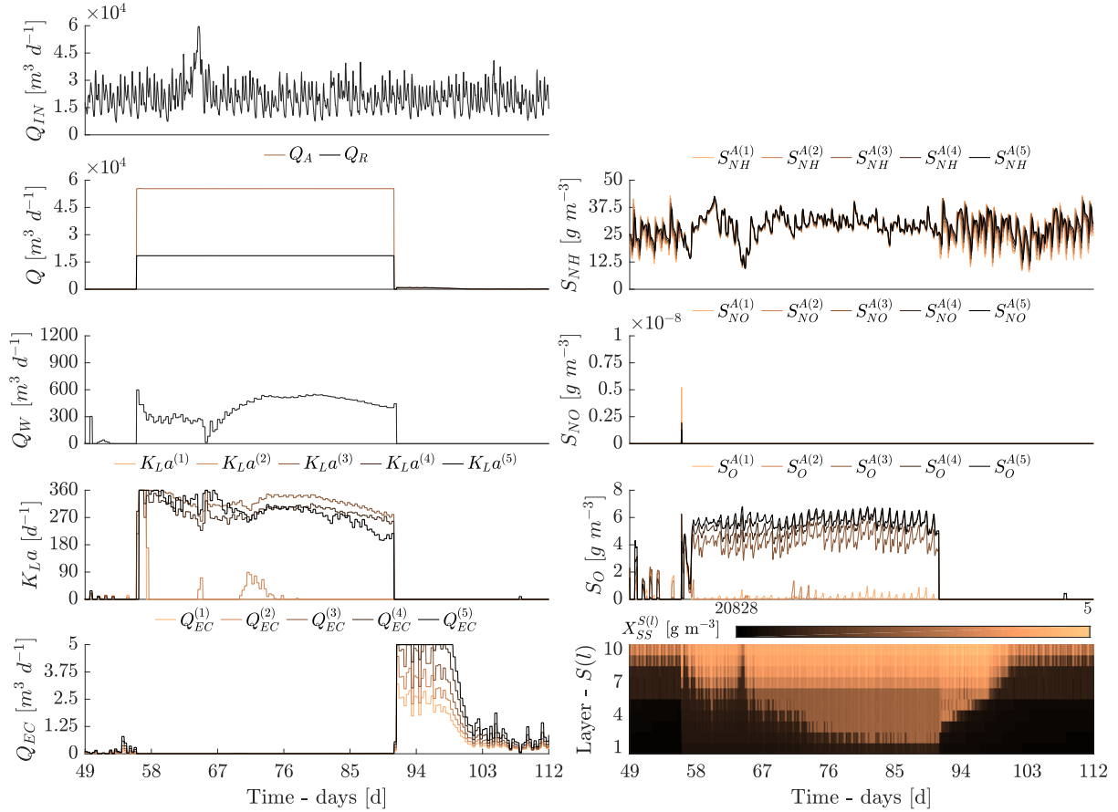
Figure 9.7: Case II, t \in [49, 112] : Influent flow-rate Q_{IN} , flow-rates ( Q_A, Q_R, Q_W ), oxygen transfer coefficients K_L a^{(1 \sim 5)} , and extra carbon flow-rates Q_{EC}^{(1 \sim 5)} , left panels, together with nitrogen forms S_{NH}^{A(1 \sim 5)} and S_{NO}^{A(1 \sim 5)} , soluble oxygen S_O^{A(1 \sim 5)} , and total suspended solids X_{SS}^{S(1 \sim 10)} , right panels.
