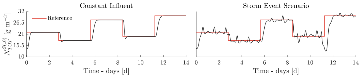
Figure 9.1: Reuse, MPC: Reference tracking of effluent total nitrogen, N_{TOT}^{S(10)} .
