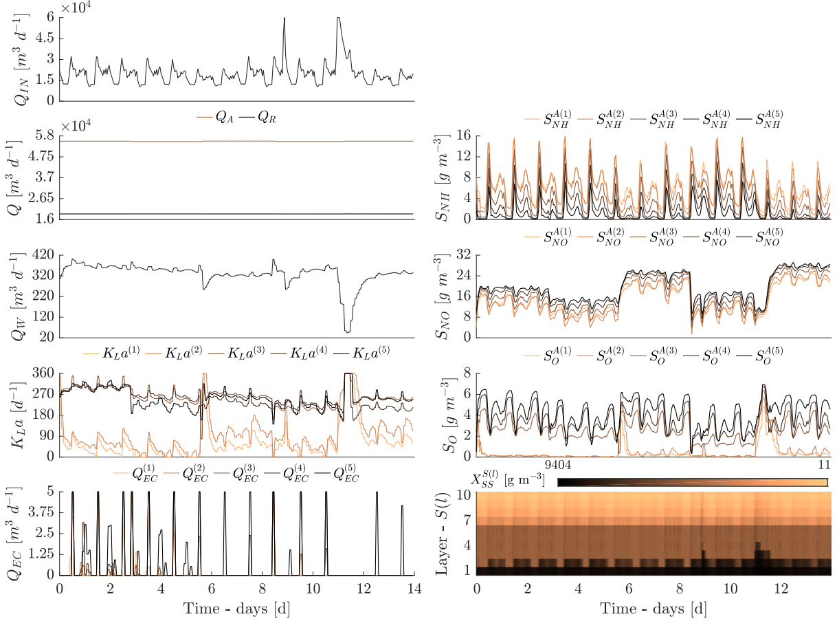
Figure 9.2: Reuse, MPC: Influent flow-rate Q_{IN} , flow-rates ( Q_A, Q_R, Q_W ), oxygen transfer coefficients K_{La}^{(1\sim 5)} , and extra carbon flow-rates Q_{EC}^{(1\sim 5)} , left panels, together with nitrogen forms S_{NH}^{A(1\sim 5)} and S_{NO}^{A(1\sim 5)} , soluble oxygen S_O^{A(1\sim 5)} , and total suspended solids X_{SS}^{S(1\sim 10)} , right panels.
